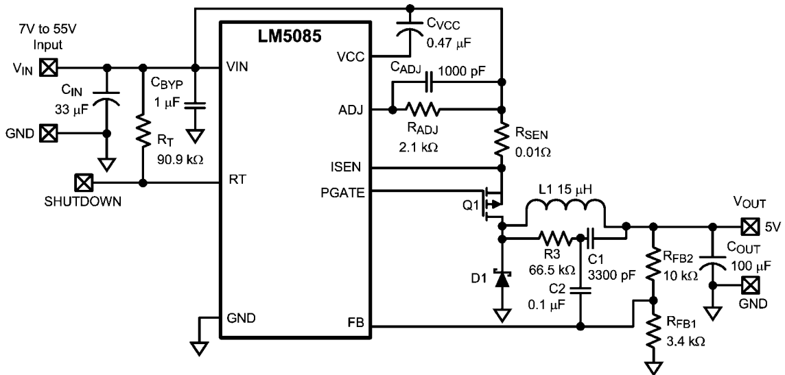
FIGURE 4. Example Circuit
